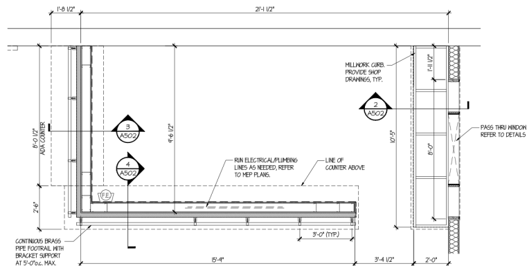
2 Enlarged Bar Plan
